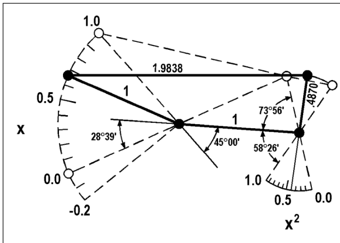
Fig. 6. Sixth-Order Approximation for Squaring Function.
