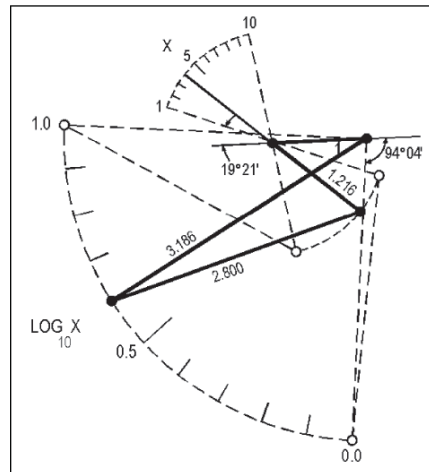
Fig. 4. Five-Point Approximation for Log Function.
