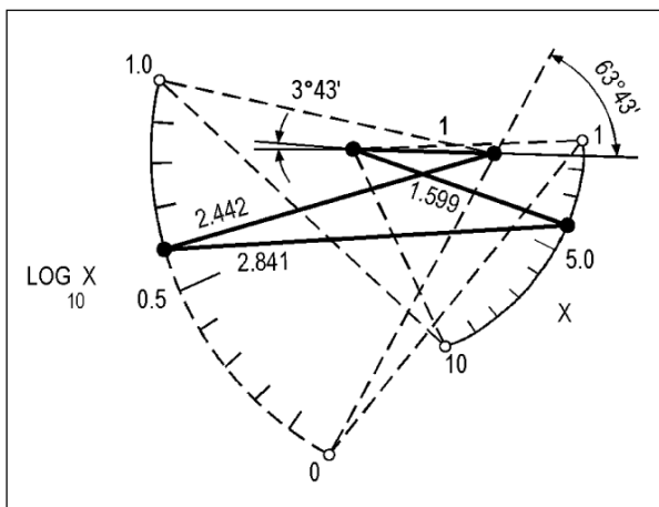
Fig. 3. Four-Point Approximation for Log Function.
