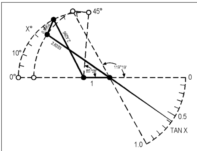
Fig. 7. Seventh-Order Approximation for Tangent Function.
