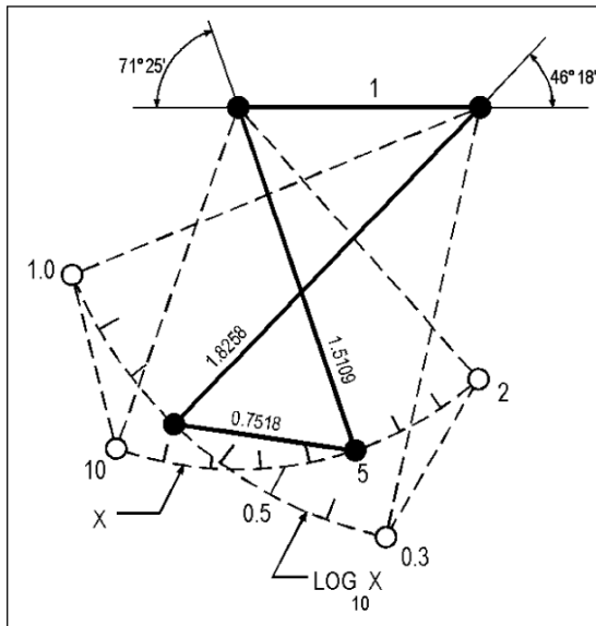
Fig. 5. Fifth-Order Approximation for Log Function.
