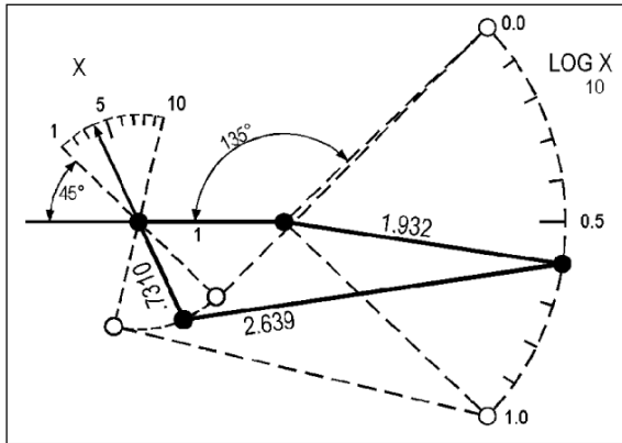
Fig. 2. Three-Point Approximation for Log Function.
